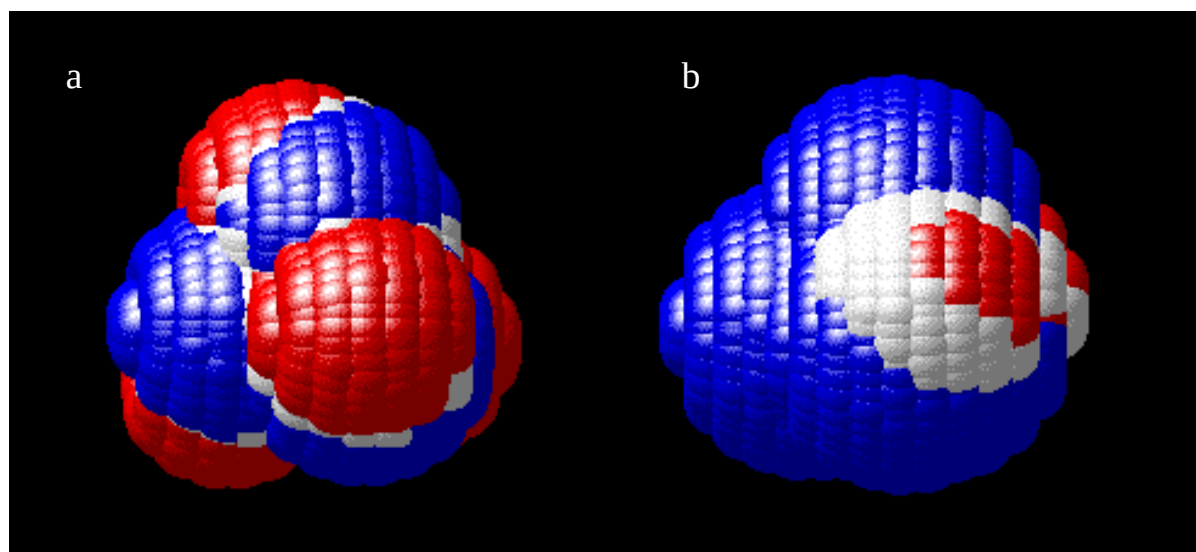
Figure 2. Charge distribution of solvent accessible surfaces of (a) Si(OH) 4 and (b) Si(OH) 3 O - molecules. Blue=positive charge, neutral=white, red=negative.
