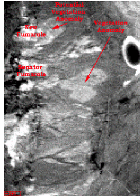
Figure 4. MNF processed AVIRIS image.
