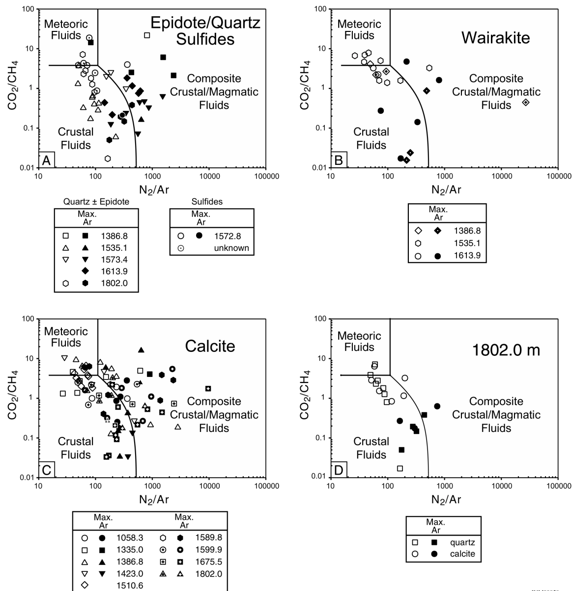
Figure 3. Plots of \text{CO}_2/\text{CH}_4 vs. \text{N}_2/\text{Ar} of inclusion fluids. Sample depths are shown in meters. Max. Ar = calculated maximum argon content. (from Norman and Moore, 1999).
