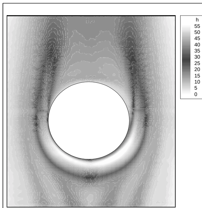
Figure 2. Measured fin-surface heat transfer coefficient, h ( \text{W/m}^2 \cdot \text{K} ), around a circular tube, flow velocity 2.8 m/s.
