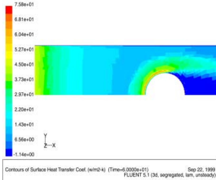
Figure 5. Modeling results for heat transfer coefficient on the fin surface of a circular tube corresponding to the experimental data in Figure 1.
