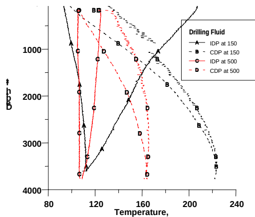
Figure 1 -- Comparison of drilling fluid temperatures in Imperial Valley field test
