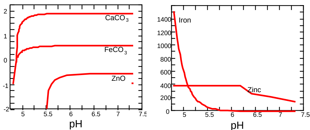
Figure 3. Results of modeling calculation of the effects of adding \text{Na}_2\text{CO}_3 to the brine to raise pH and induce mineral precipitation. The concentration of iron is selectively lowered due to iron carbonate precipitation until just above pH 5.5 where zinc oxide begins to precipitate. Calcite (calcium carbonate) also precipitates as the pH rises. Calculations performed using the React code (Bethke, 1992).
