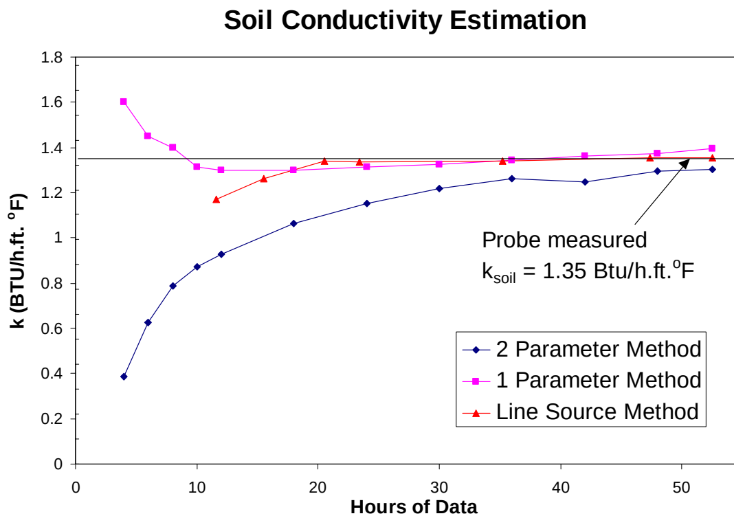
Figure 4. Results of soil thermal conductivity estimates using test data of different duration. Three sets of results are compared with the independently measured value, (a) the numerical two-parameter method (Austin 1998), (b) a one-parameter estimation method, and (c) the line-source method results (Smith 1999a).
