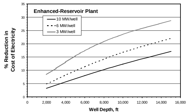
Figure 2. % Reduction in the Cost of Electricity for 50-MW flashed-steam, binary, and enhanced-reservoir geothermal power plants, assuming a 25% reduction in Well Costs, a 25% reduction in the Dry Well Rate, and a 25% increase in Average Well Productivity.
