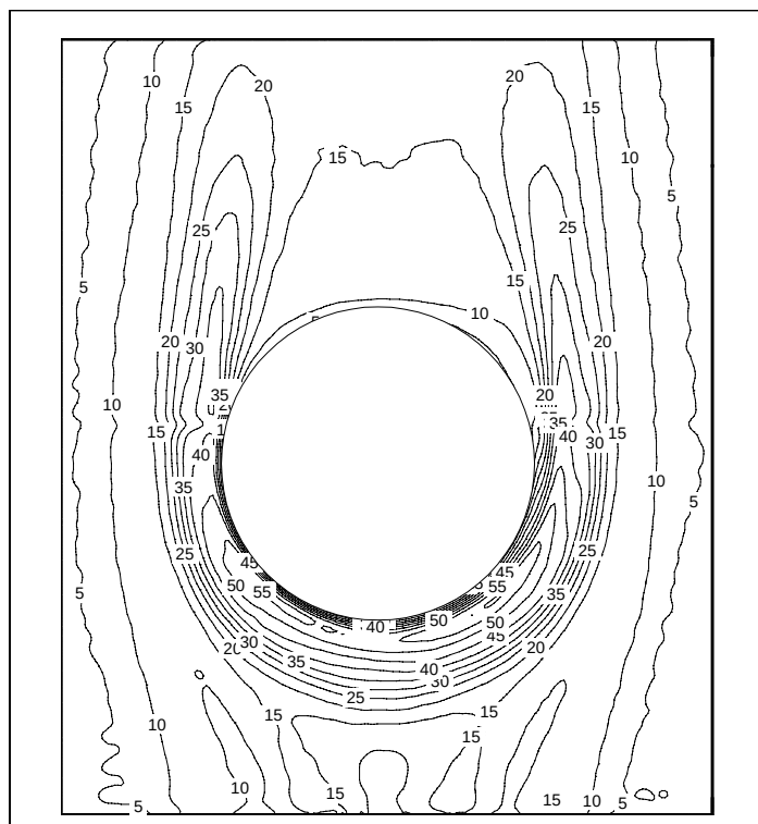
Figure 1. The contours represent measured values of local fin-surface heat transfer coefficient in \text{W/m}^2 \cdot \text{K} for flow around a circular tube in a simulated fin/tube flow passage. Flow is from bottom to top in the figure with a mean velocity of 2.8 m/s.
